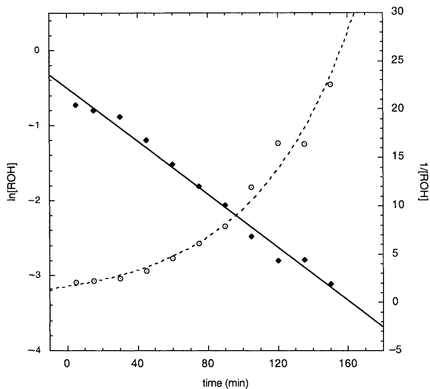
Figure 1. Plot of ln[ROH] (◆) and 1/[ROH] (○) versus time for the etherification of benzhydrol by [{(R,R)-diop}PdCl 2 ]/2AgOTf; conditions: [ROH] = 0.50 M, [{(R,R)-diop}PdCl 2 ] = 0.01 M, and [AgOTf] = 0.02 M in CH 3 NO 2 at 50 °C
